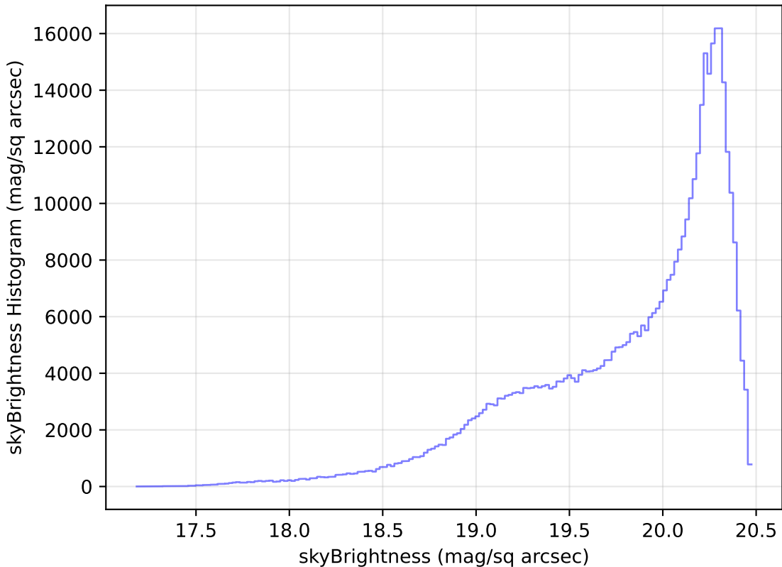
ddf_half_v3.4_10yrs All sky i band: skyBrightness Histogram
