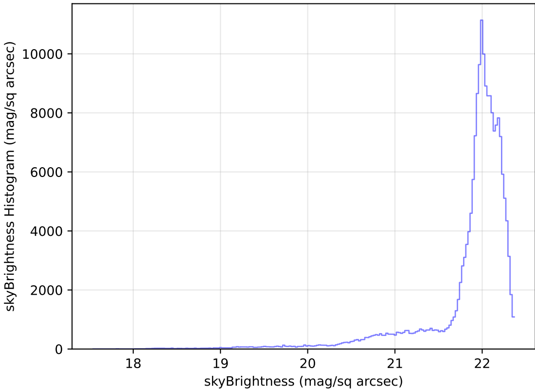
ddf_half_v3.4_10yrs All sky g band: skyBrightness Histogram
