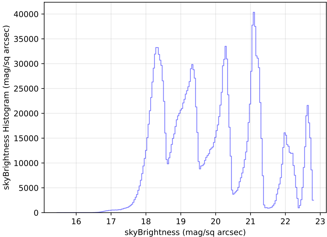
ddf_half_v3.4_10yrs All sky all bands: skyBrightness Histogram
