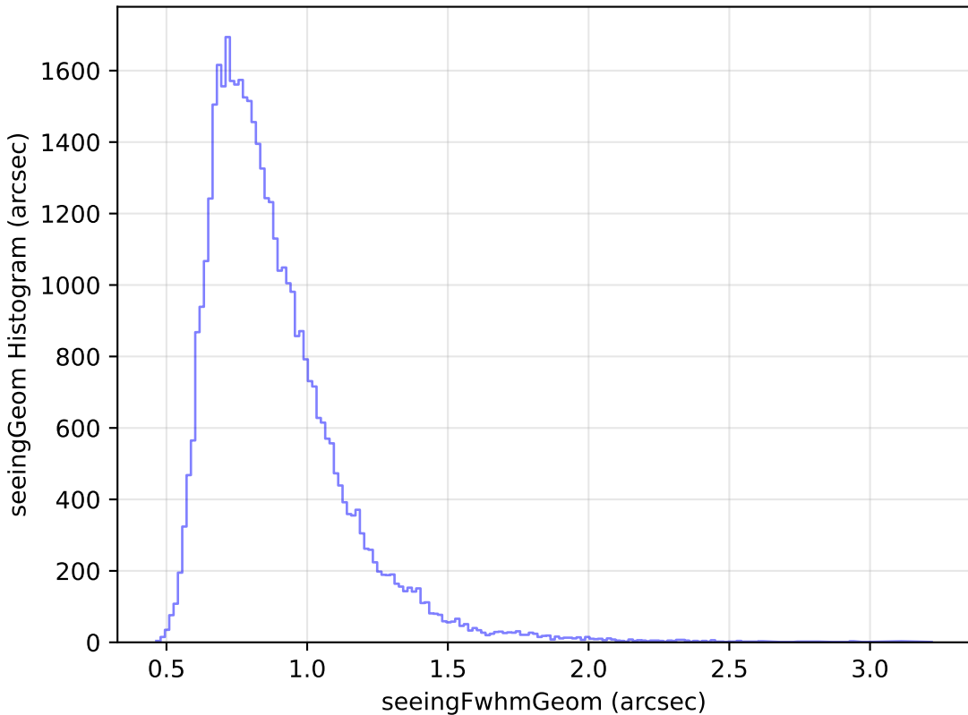
ddf_half_v3.4_10yrs Yr 1 z band: seeingGeom Histogram
