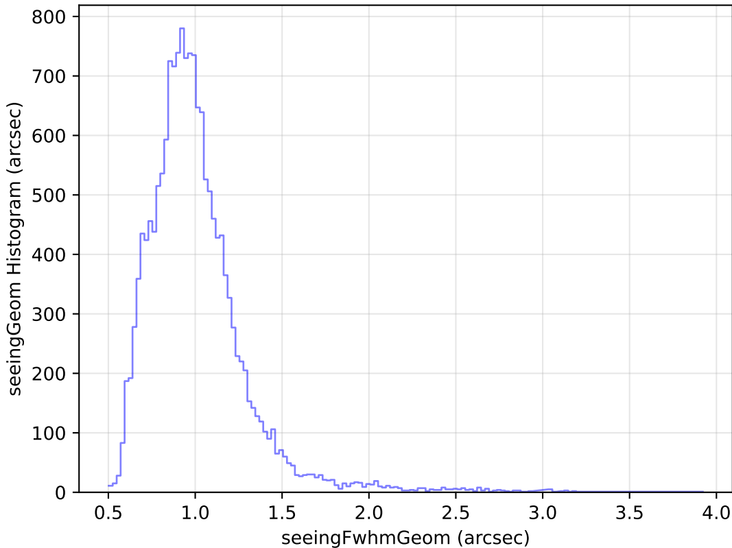
ddf_half_v3.4_10yrs Yr 1 u band: seeingGeom Histogram
