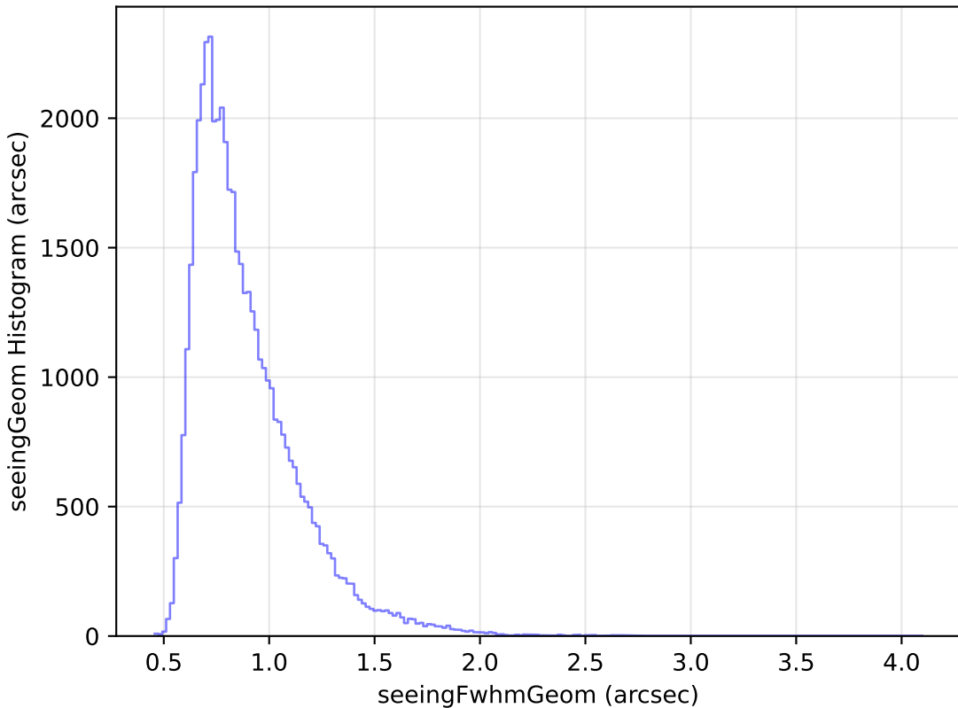
ddf_half_v3.4_10yrs Yr 1 r band: seeingGeom Histogram
