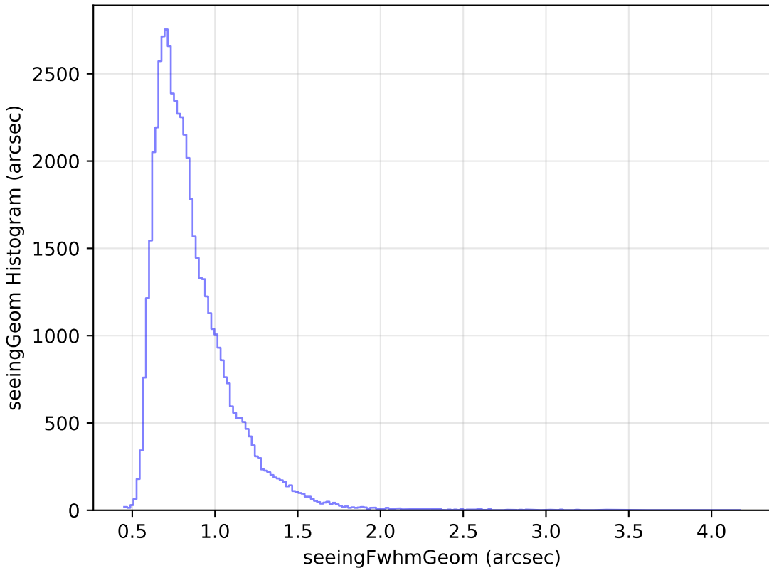
ddf_half_v3.4_10yrs Yr 1 i band: seeingGeom Histogram
