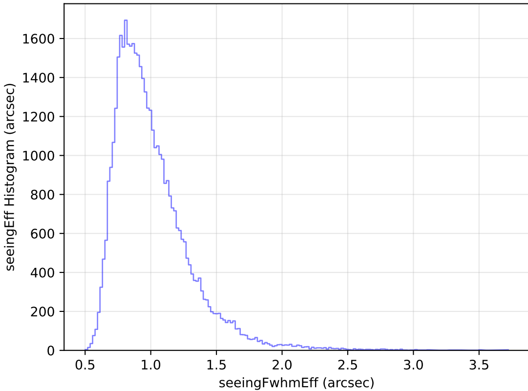
ddf_half_v3.4_10yrs Yr 1 z band: seeingEff Histogram
