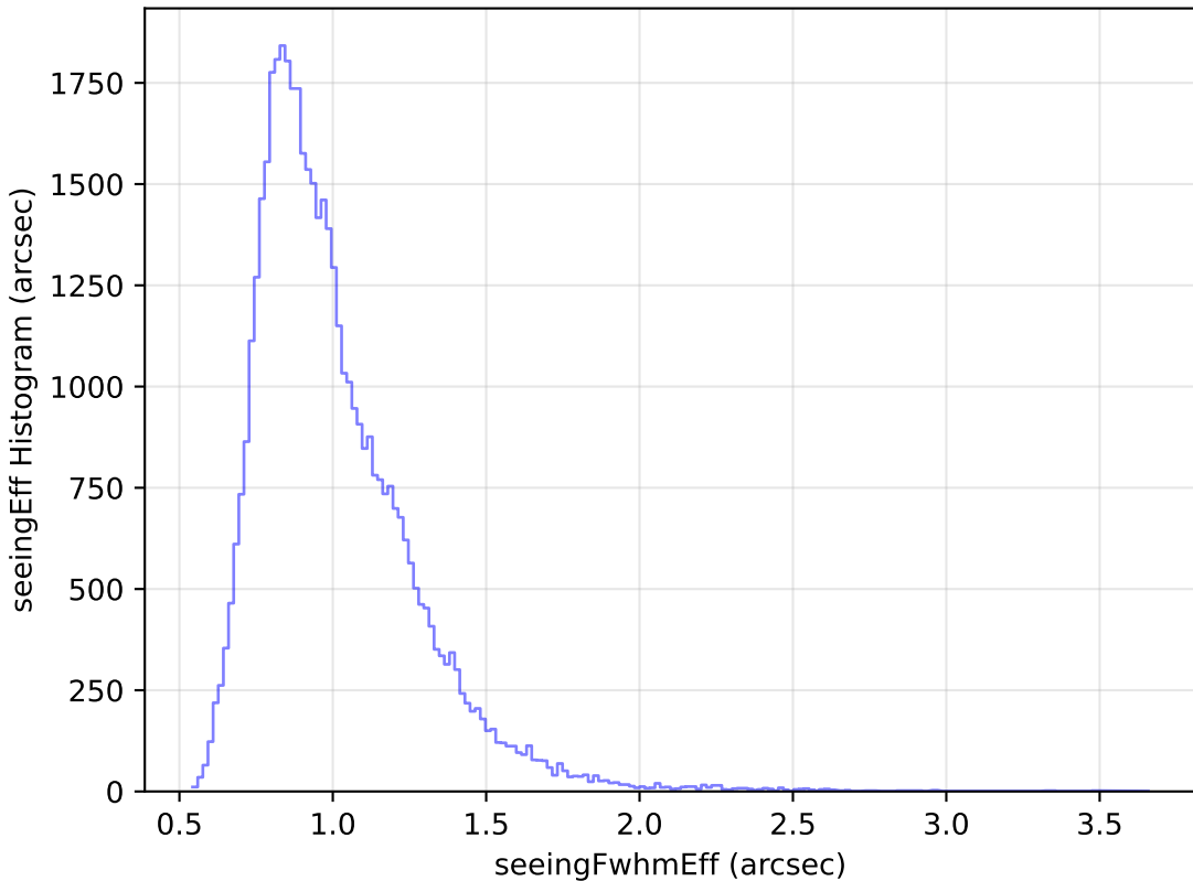
ddf_half_v3.4_10yrs Yr 1 y band: seeingEff Histogram
