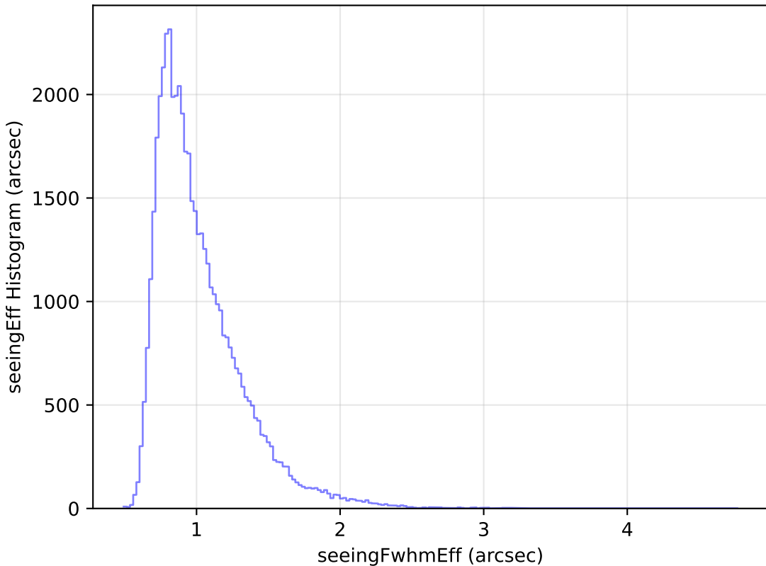
ddf_half_v3.4_10yrs Yr 1 r band: seeingEff Histogram
