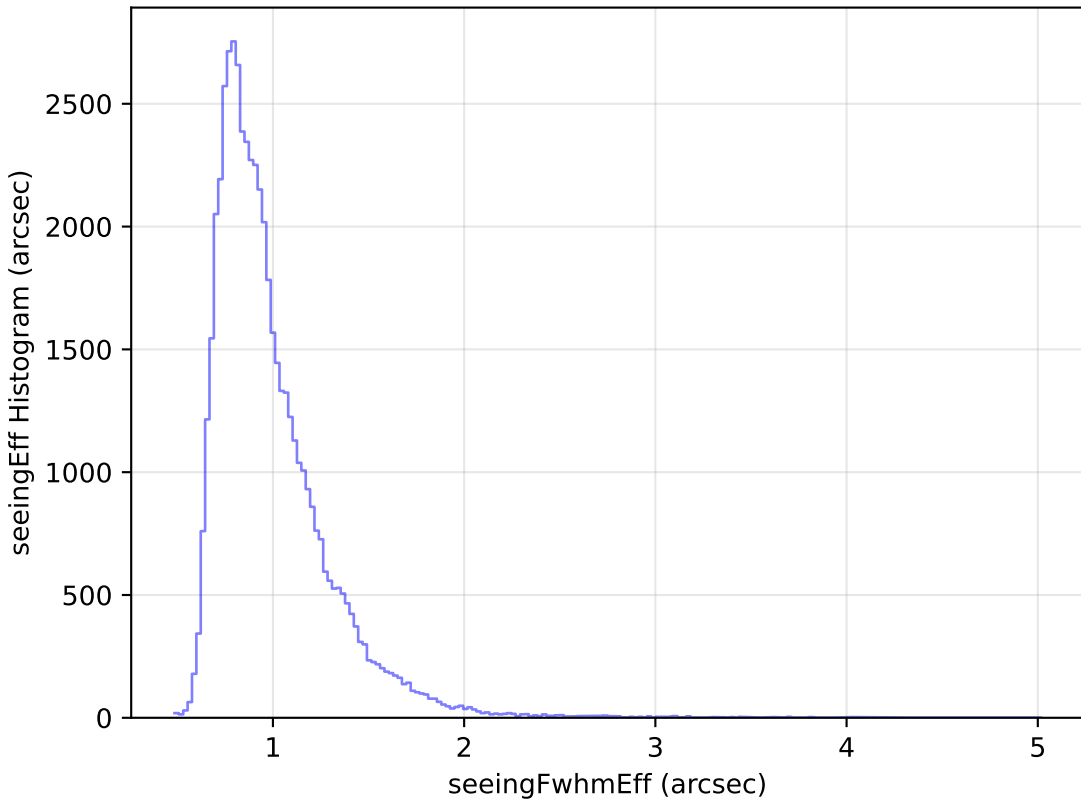
ddf_half_v3.4_10yrs Yr 1 i band: seeingEff Histogram
