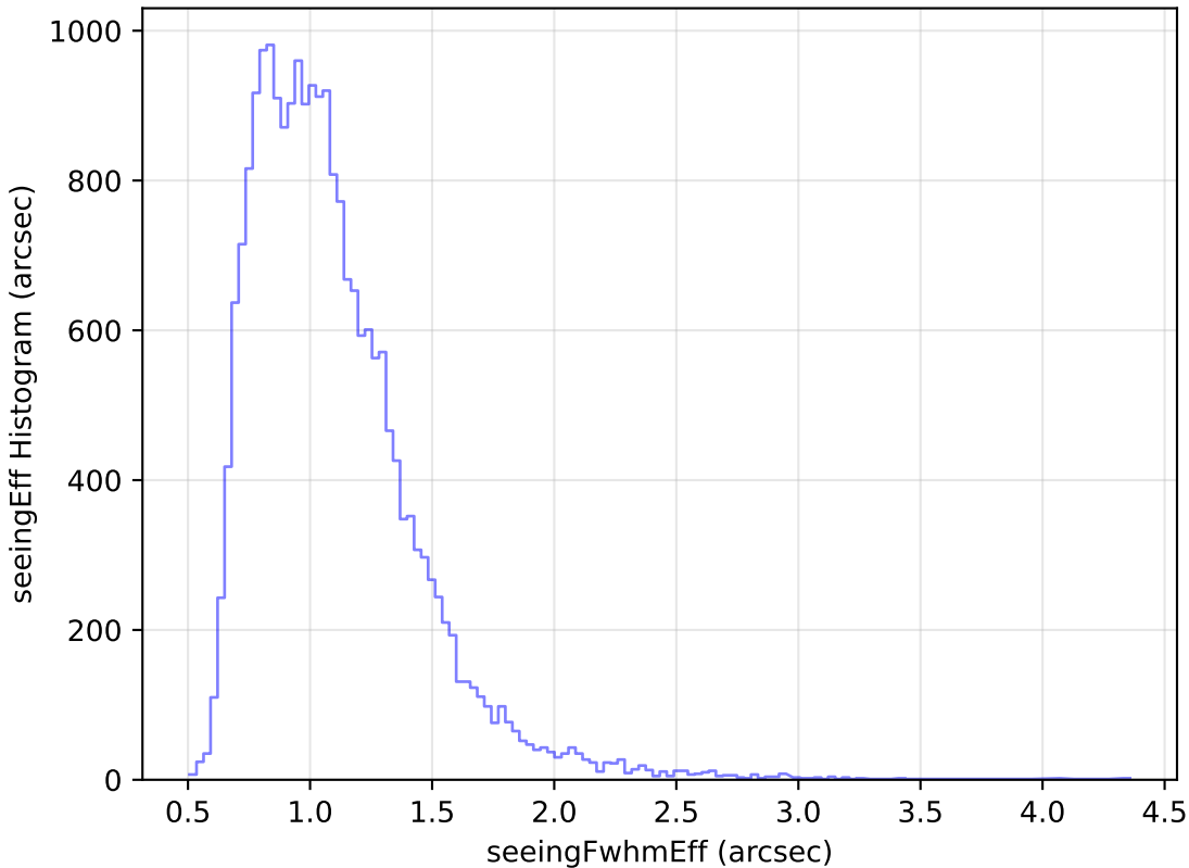
ddf_half_v3.4_10yrs Yr 1 g band: seeingEff Histogram
