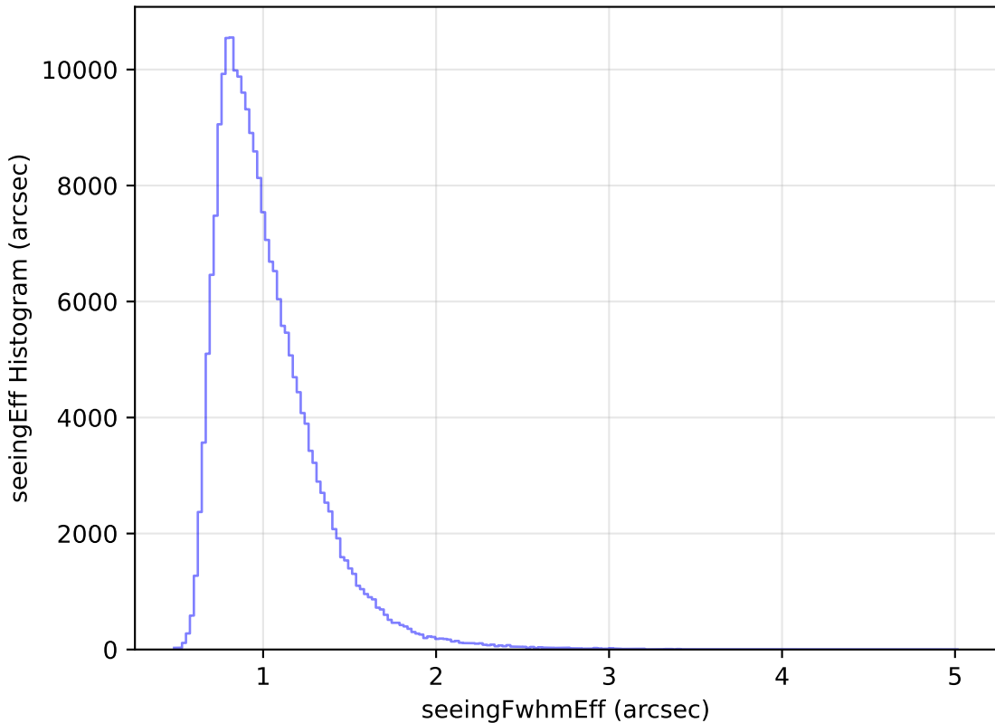
ddf_half_v3.4_10yrs Yr 1 all bands: seeingEff Histogram
