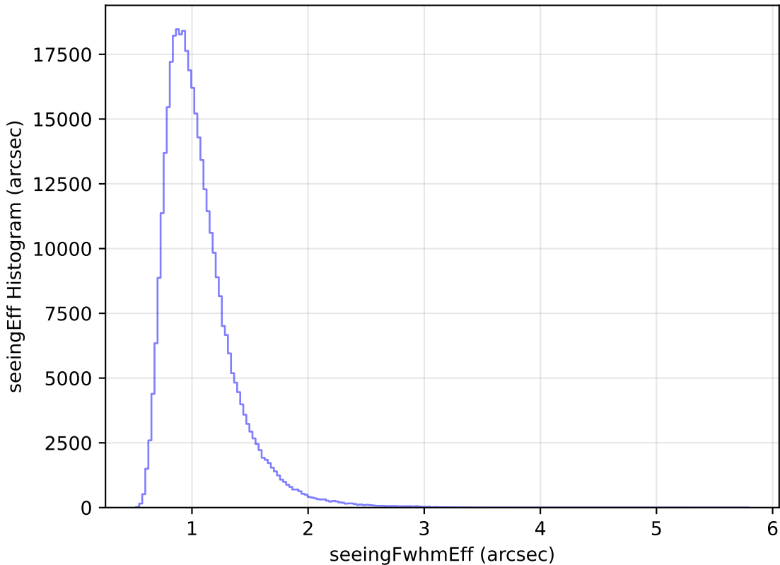
ddf_half_v3.4_10yrs WFD y band: seeingEff Histogram
