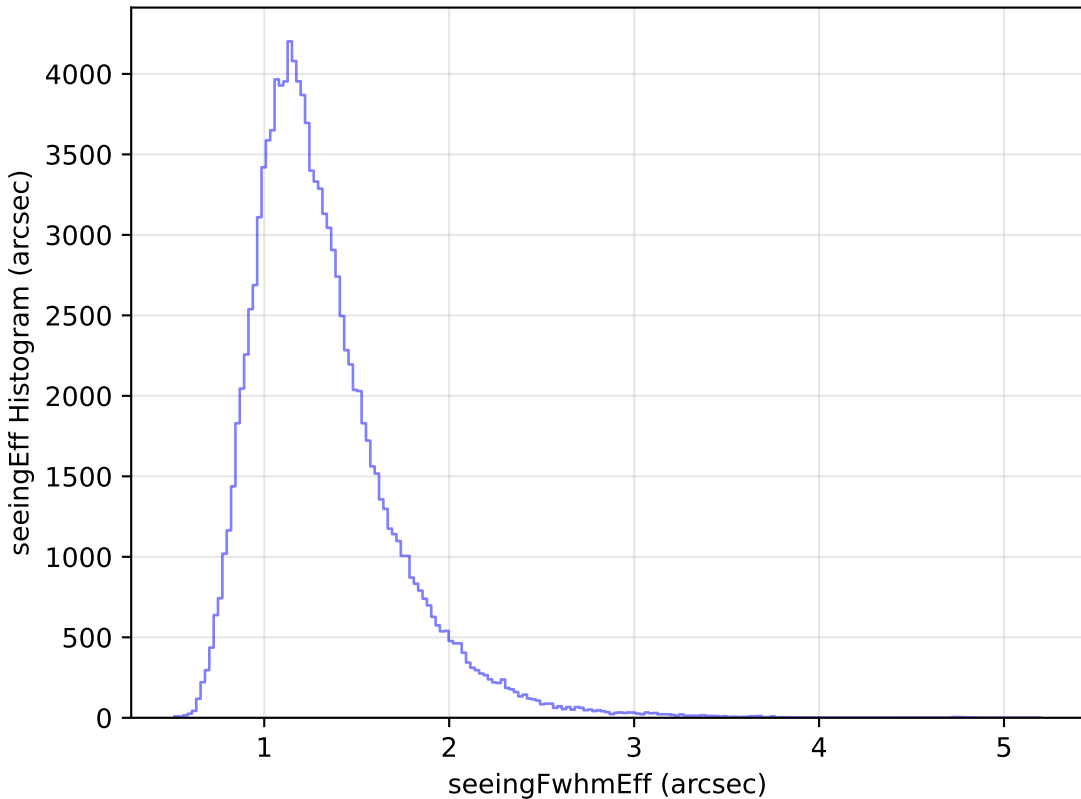
ddf_half_v3.4_10yrs WFD u band: seeingEff Histogram
