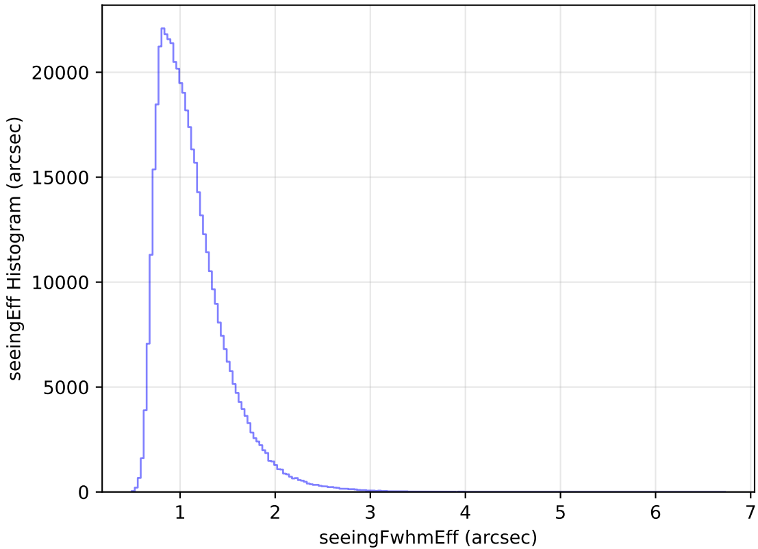
ddf_half_v3.4_10yrs WFD r band: seeingEff Histogram
