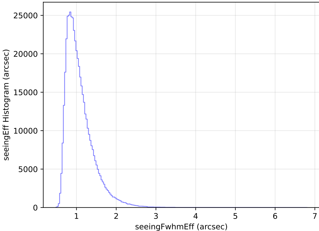
ddf_half_v3.4_10yrs WFD i band: seeingEff Histogram
