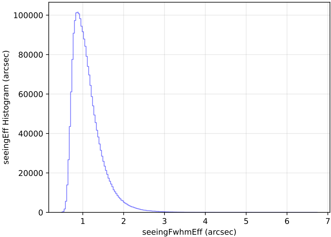
ddf_half_v3.4_10yrs WFD all bands: seeingEff Histogram
