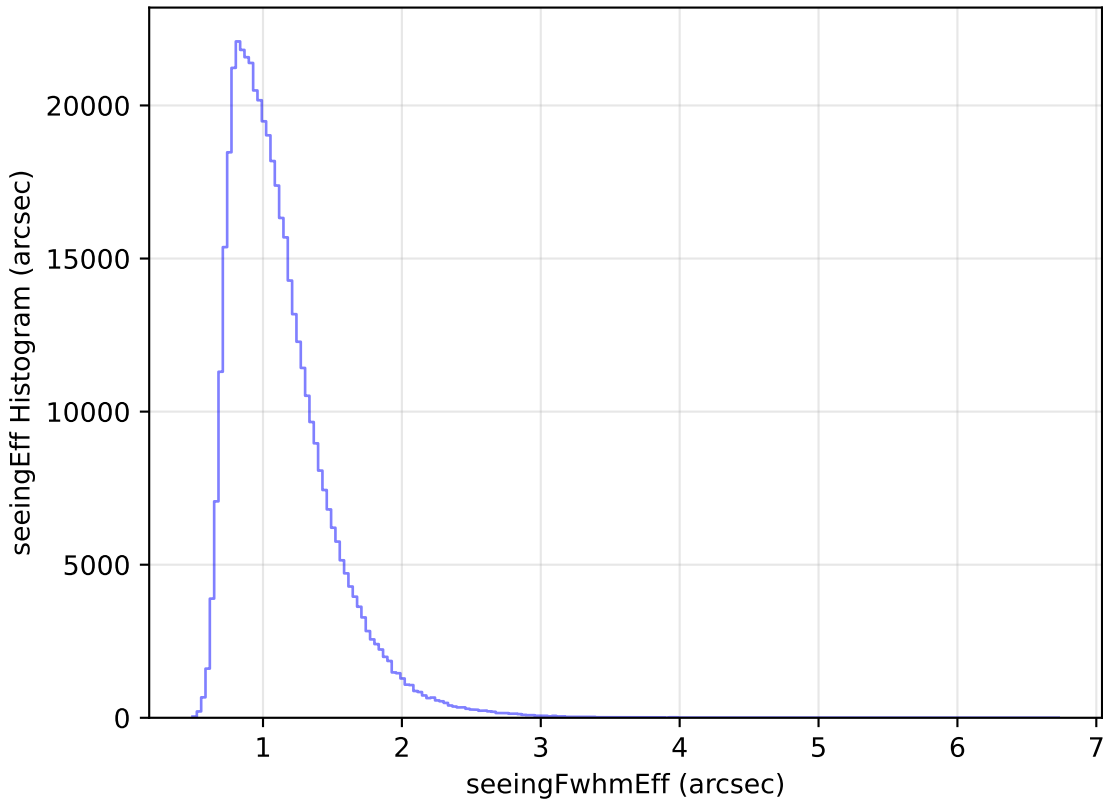
ddf_half_v3.4_10yrs All sky r band: seeingEff Histogram
