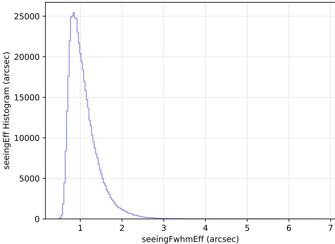
ddf_half_v3.4_10yrs All sky i band: seeingEff Histogram
