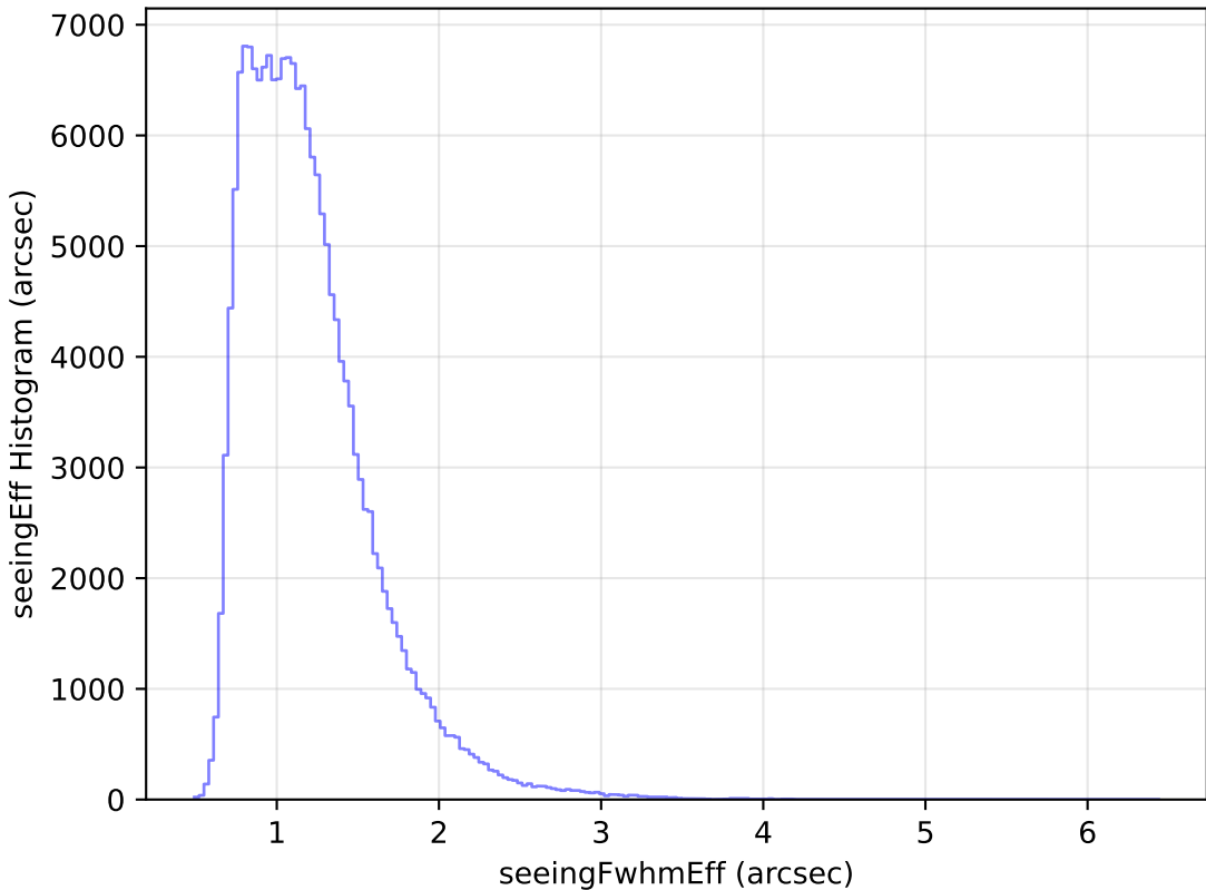
ddf_half_v3.4_10yrs All sky g band: seeingEff Histogram
