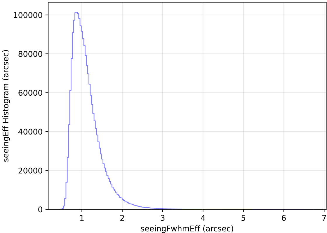
ddf_half_v3.4_10yrs All sky all bands: seeingEff Histogram
