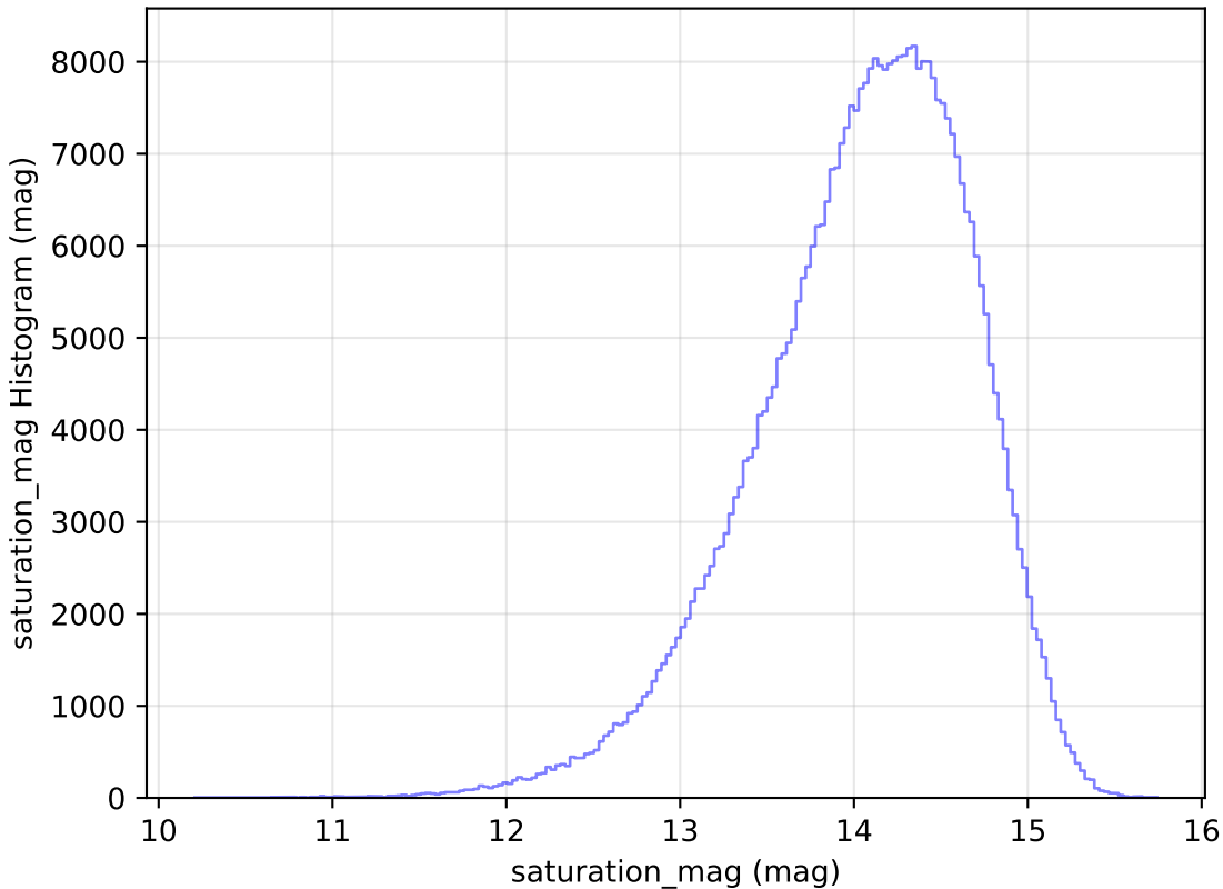
ddf_half_v3.4_10yrs WFD z band: saturation_mag Histogram
