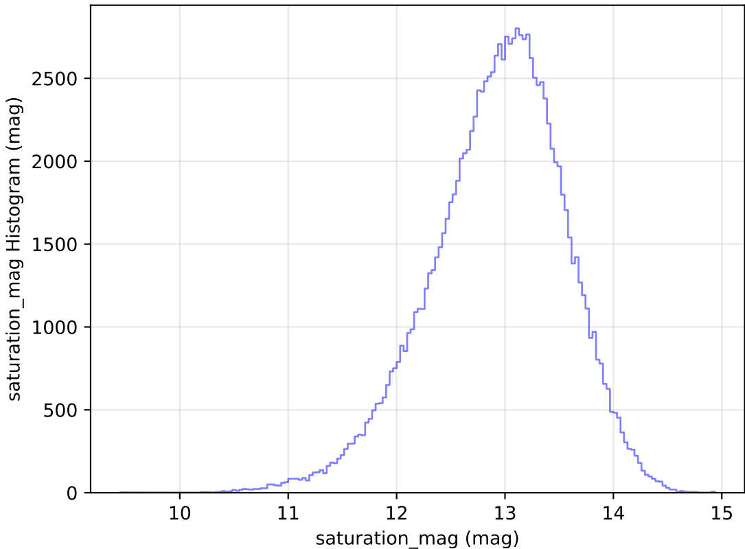
ddf_half_v3.4_10yrs WFD u band: saturation_mag Histogram
