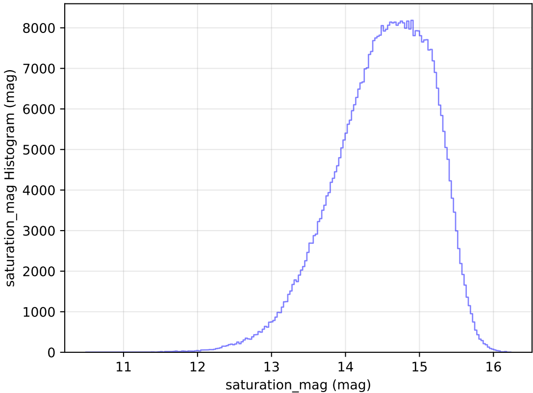
ddf_half_v3.4_10yrs WFD r band: saturation_mag Histogram
