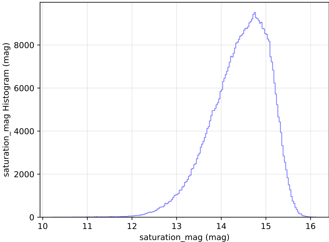
ddf_half_v3.4_10yrs WFD i band: saturation_mag Histogram
