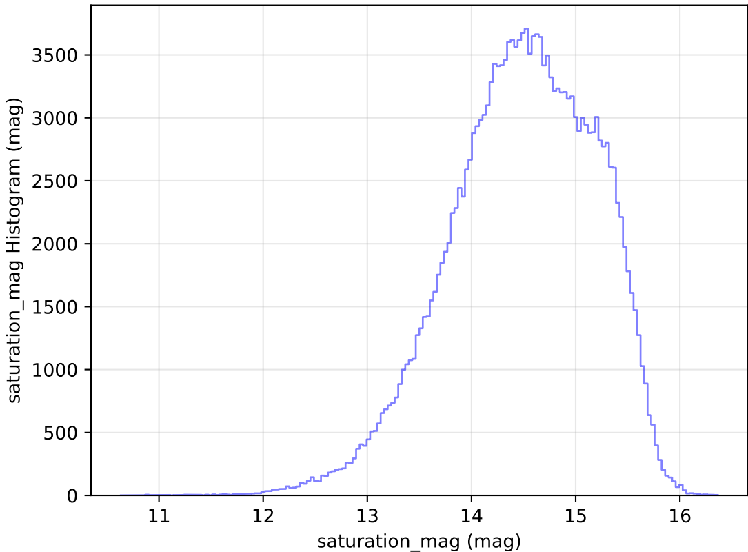
ddf_half_v3.4_10yrs WFD g band: saturation_mag Histogram
