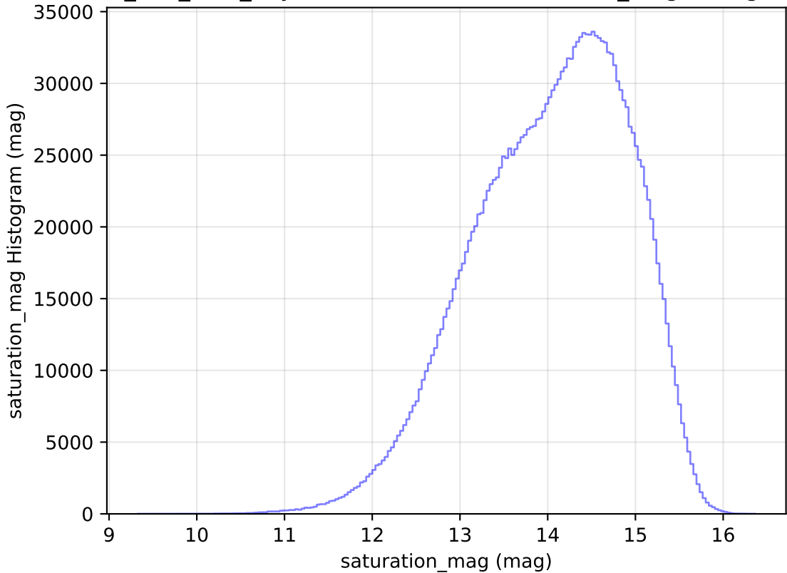
ddf_half_v3.4_10yrs WFD all bands: saturation_mag Histogram
