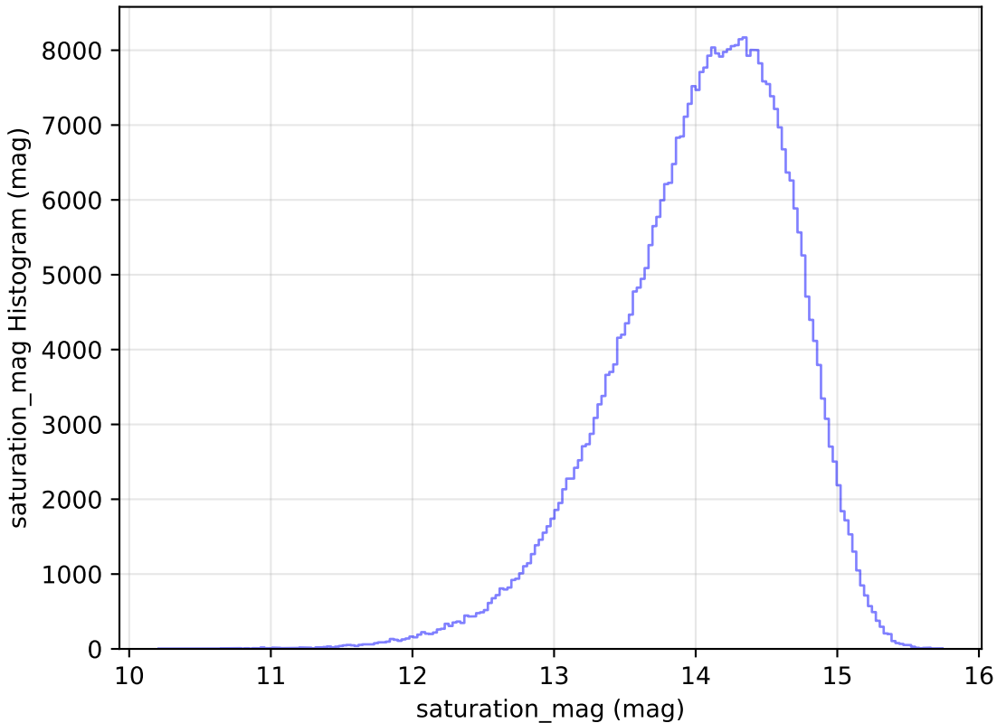
ddf_half_v3.4_10yrs All sky z band: saturation_mag Histogram
