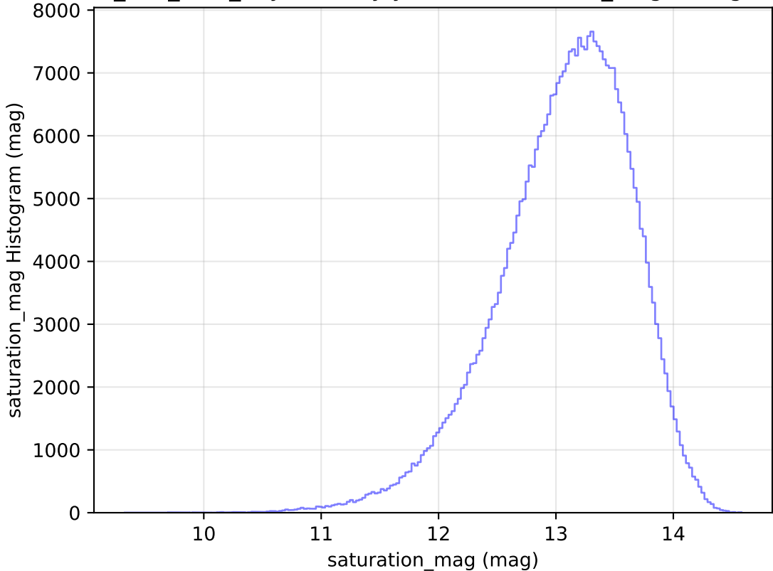
ddf_half_v3.4_10yrs All sky y band: saturation_mag Histogram
