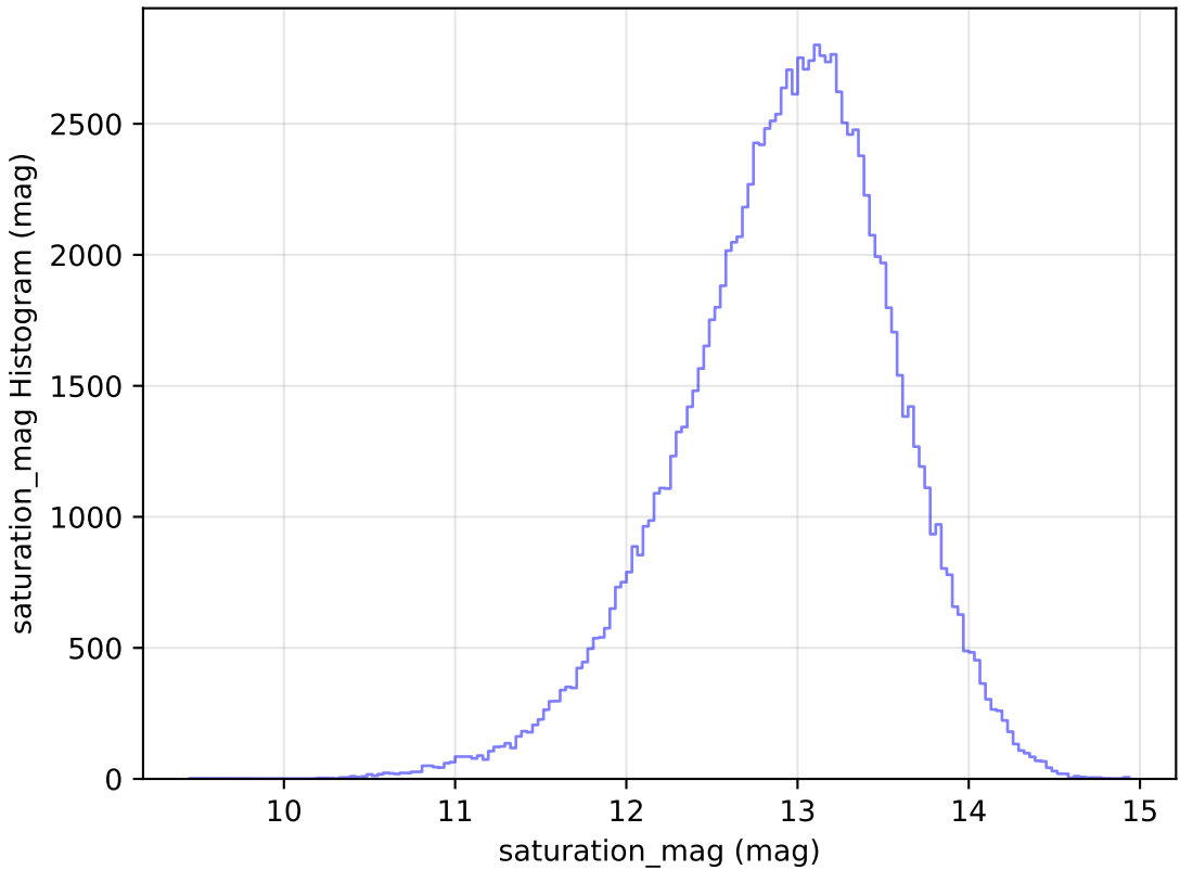
ddf_half_v3.4_10yrs All sky u band: saturation_mag Histogram
