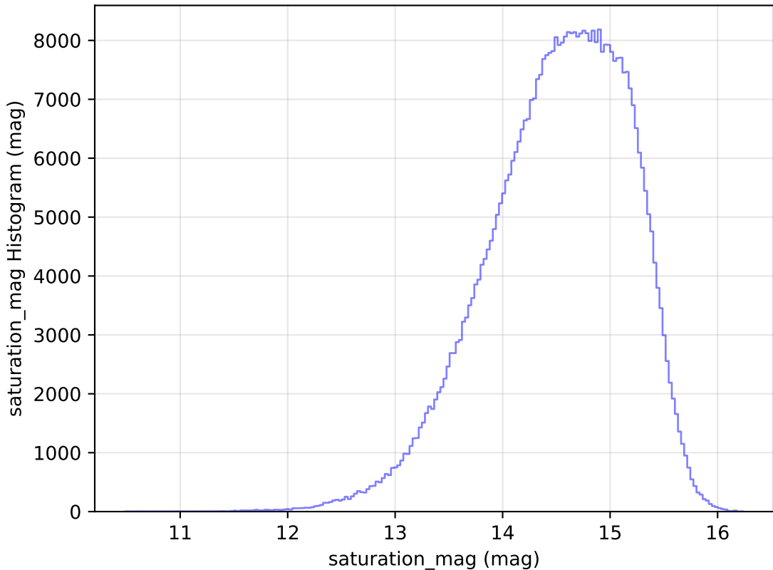
ddf_half_v3.4_10yrs All sky r band: saturation_mag Histogram
