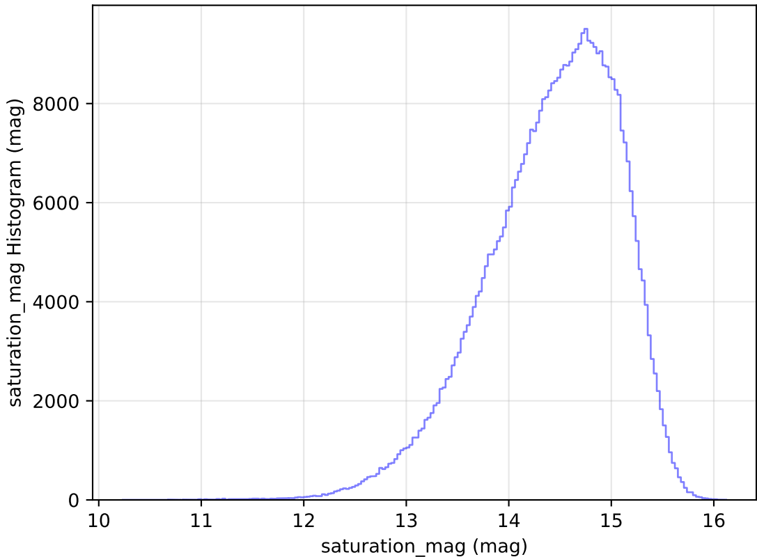
ddf_half_v3.4_10yrs All sky i band: saturation_mag Histogram
