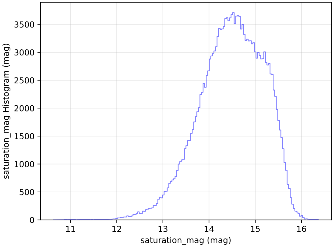
ddf_half_v3.4_10yrs All sky g band: saturation_mag Histogram
