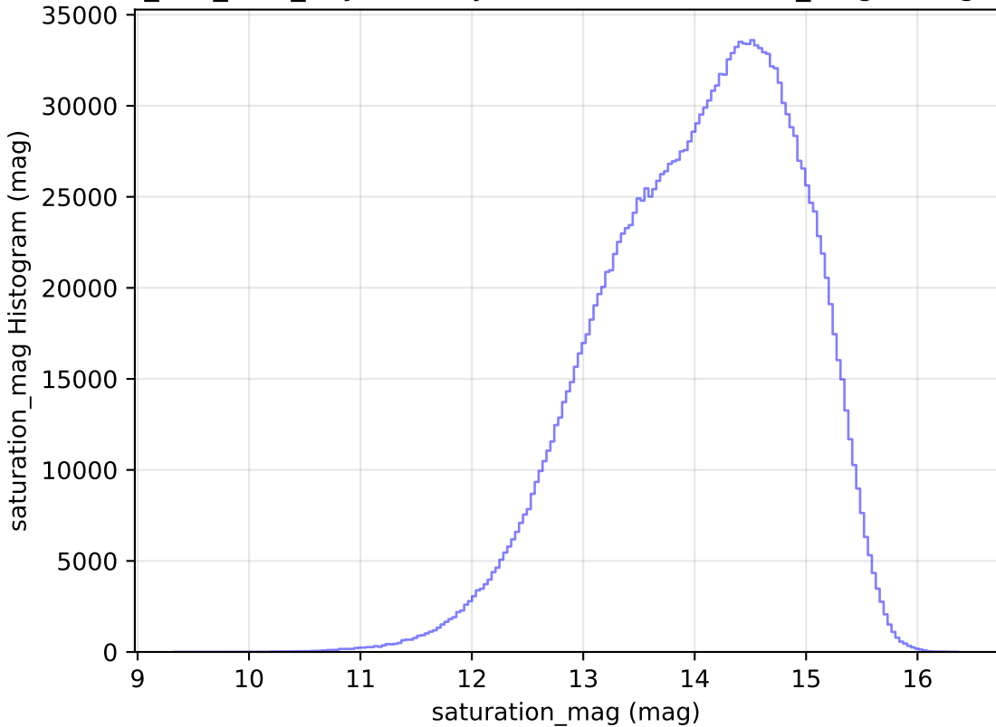
ddf_half_v3.4_10yrs All sky all bands: saturation_mag Histogram
