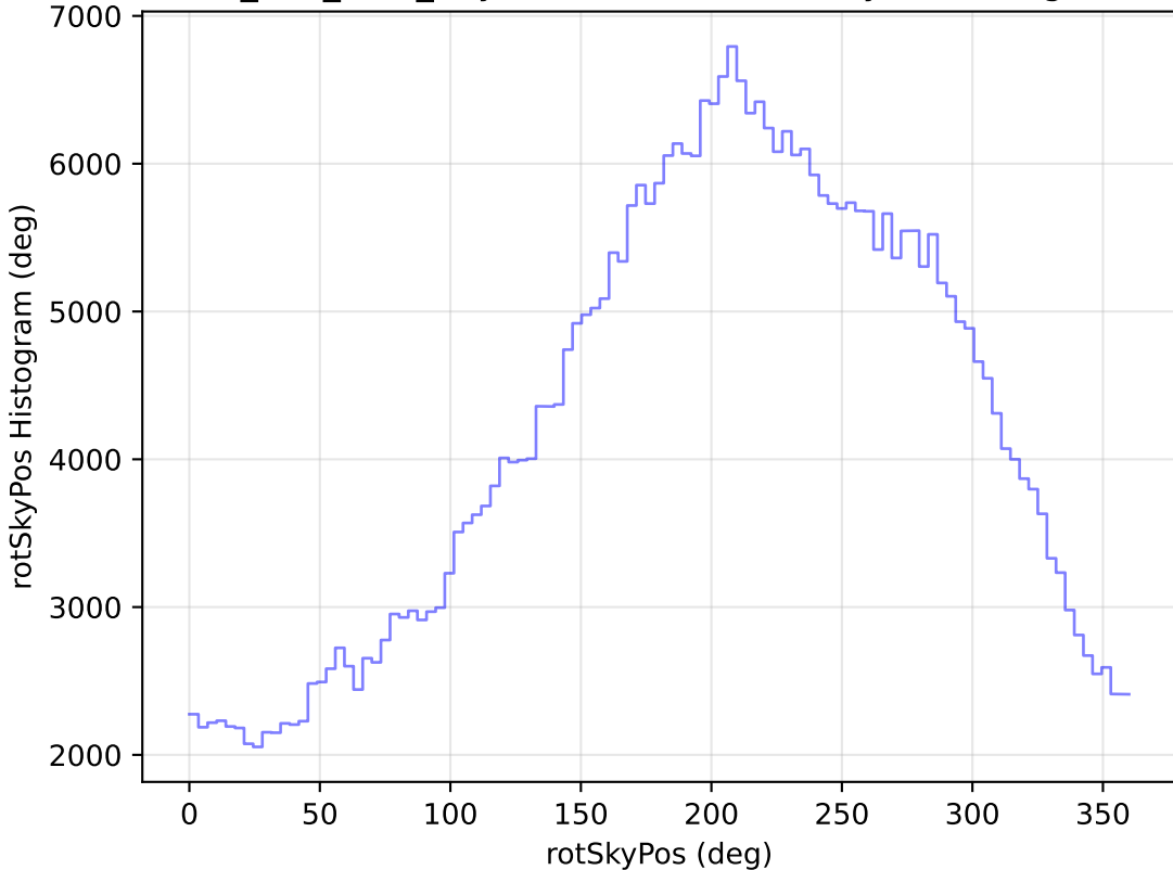
ddf_half_v3.4_10yrs WFD z band: rotSkyPos Histogram
