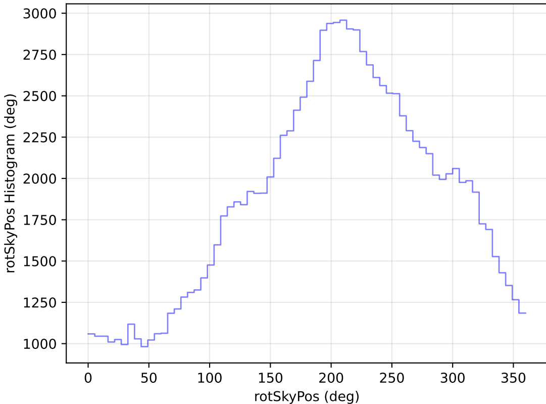
ddf_half_v3.4_10yrs WFD u band: rotSkyPos Histogram
