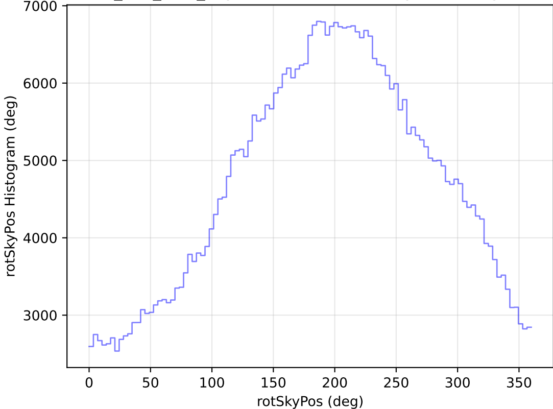
ddf_half_v3.4_10yrs WFD r band: rotSkyPos Histogram
