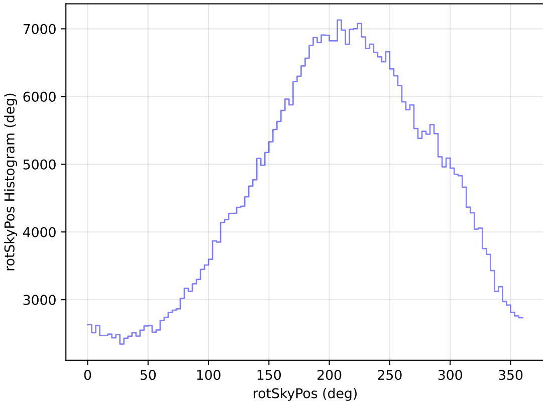
ddf_half_v3.4_10yrs WFD i band: rotSkyPos Histogram
