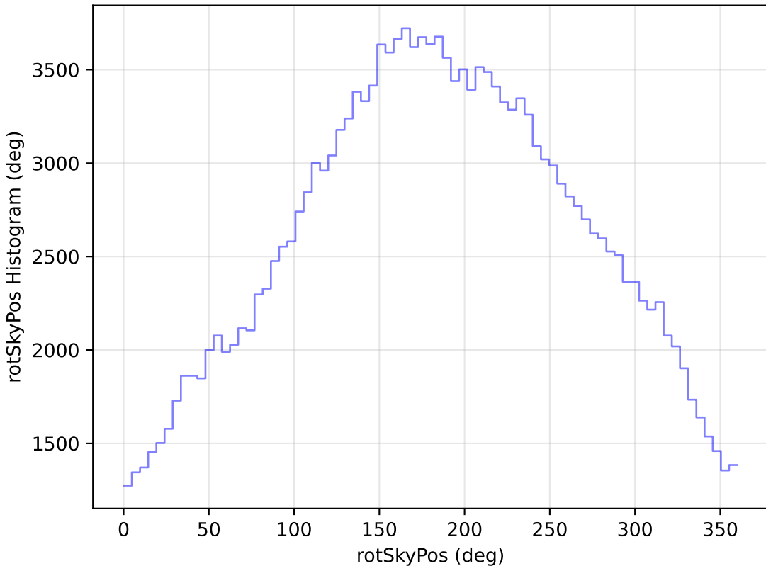
ddf_half_v3.4_10yrs WFD g band: rotSkyPos Histogram
