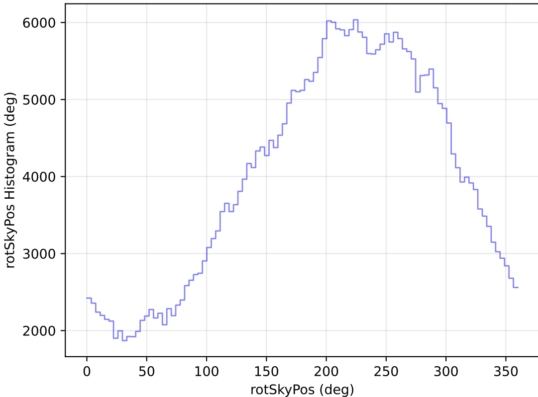
ddf_half_v3.4_10yrs All sky y band: rotSkyPos Histogram
