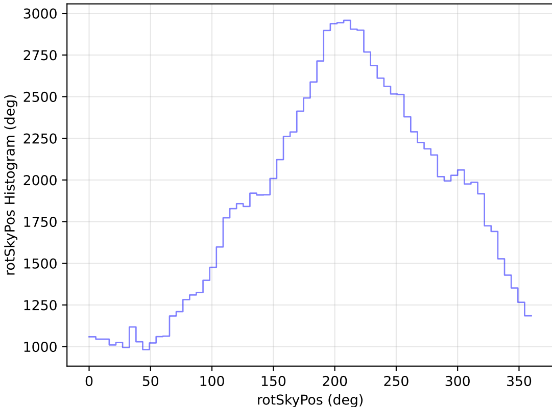
ddf_half_v3.4_10yrs All sky u band: rotSkyPos Histogram
