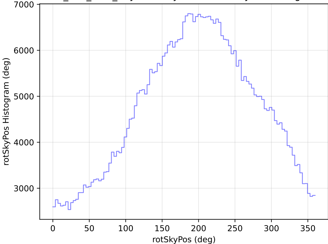
ddf_half_v3.4_10yrs All sky r band: rotSkyPos Histogram
