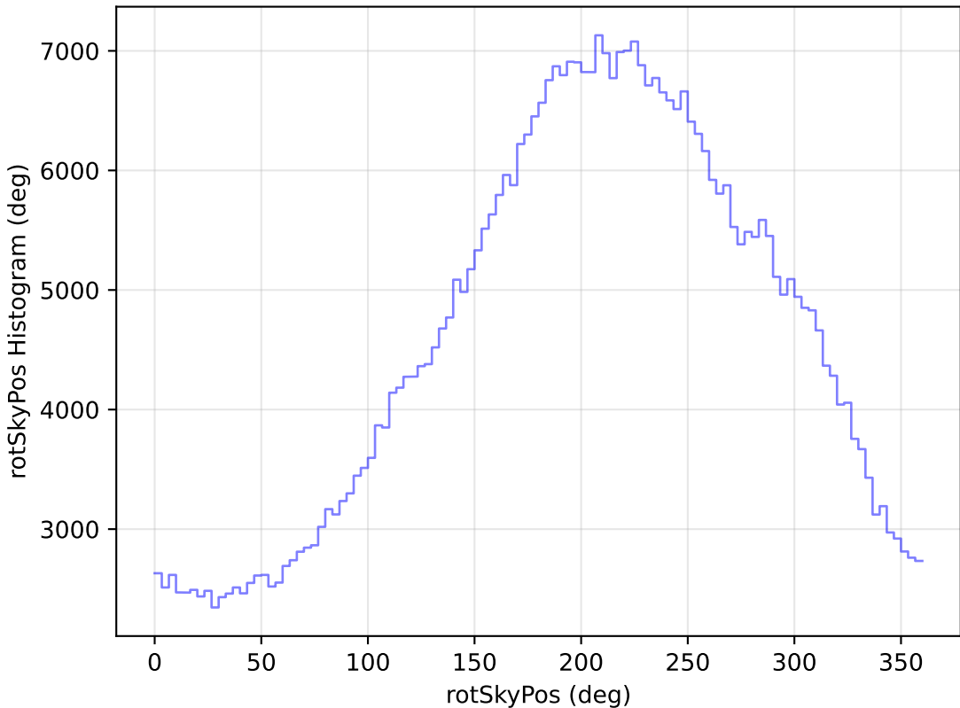
ddf_half_v3.4_10yrs All sky i band: rotSkyPos Histogram
