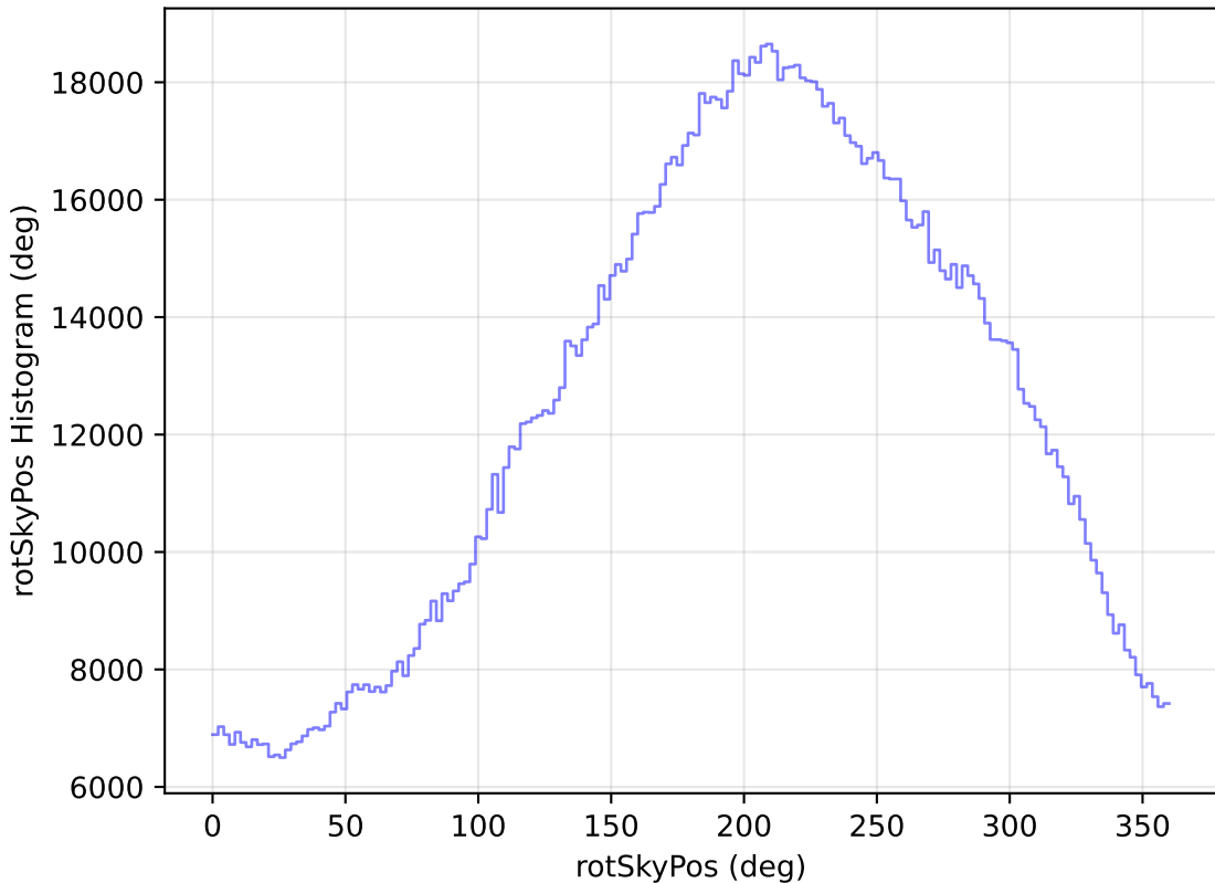
ddf_half_v3.4_10yrs All sky all bands: rotSkyPos Histogram
