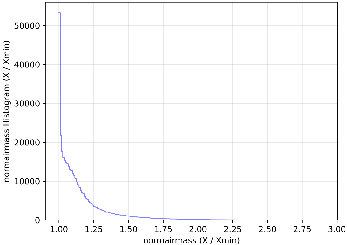
ddf_half_v3.4_10yrs WFD y band: normairmass Histogram
