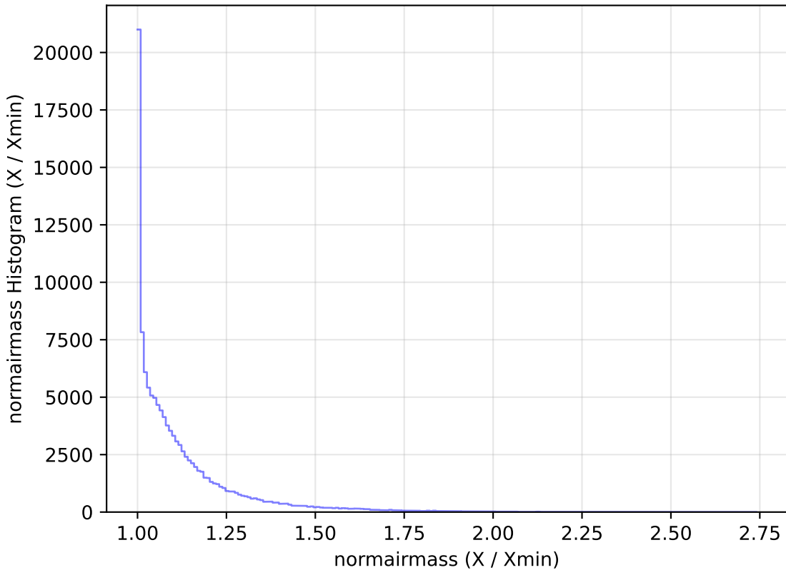
ddf_half_v3.4_10yrs WFD u band: normairmass Histogram
