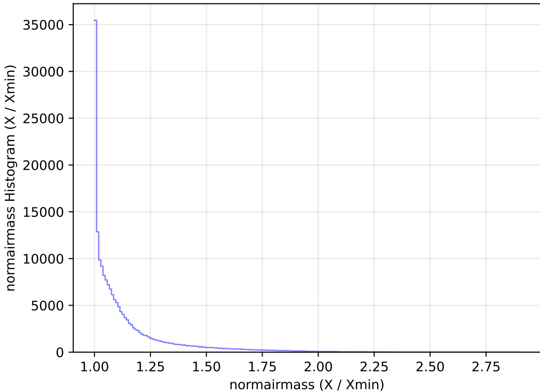
ddf_half_v3.4_10yrs WFD g band: normairmass Histogram
