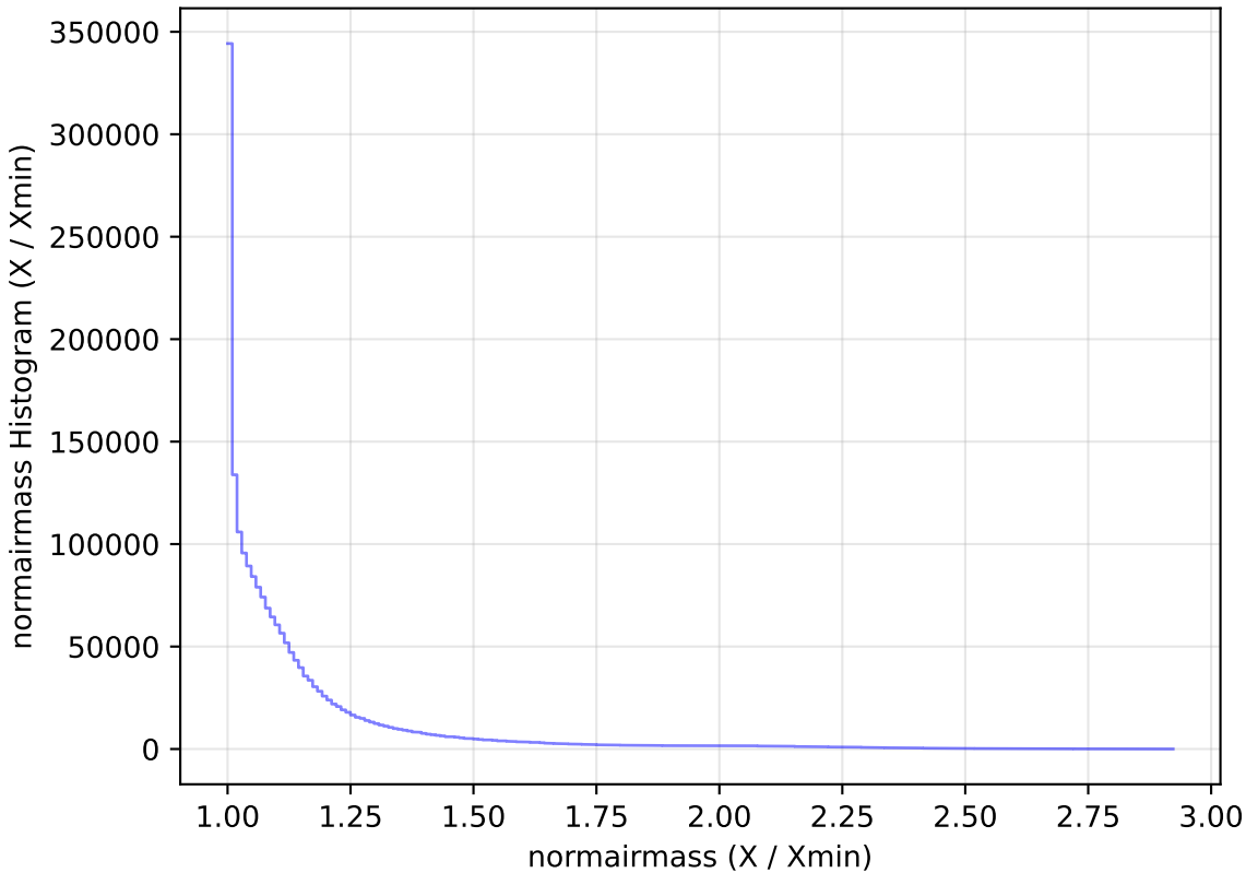
ddf_half_v3.4_10yrs WFD all bands: normairmass Histogram
