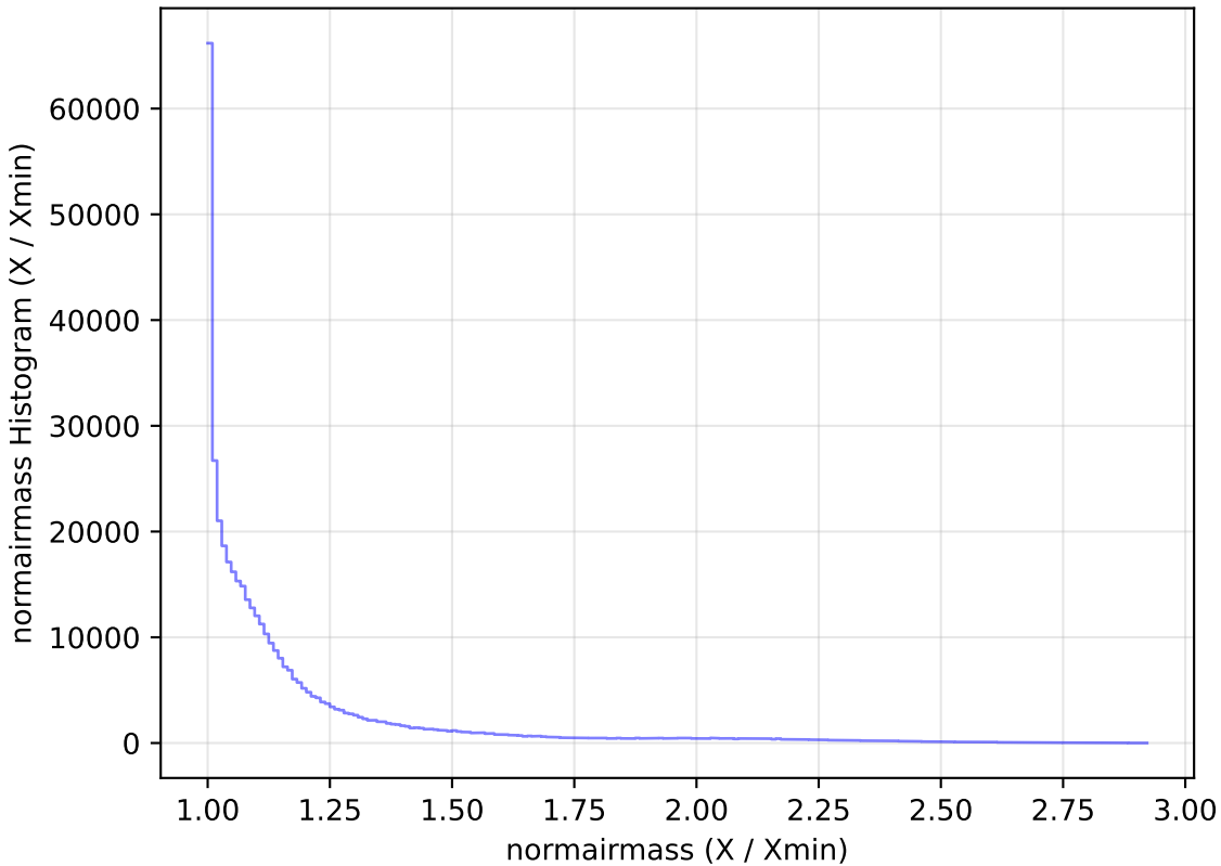
ddf_half_v3.4_10yrs All sky z band: normairmass Histogram
